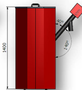
340 literes
